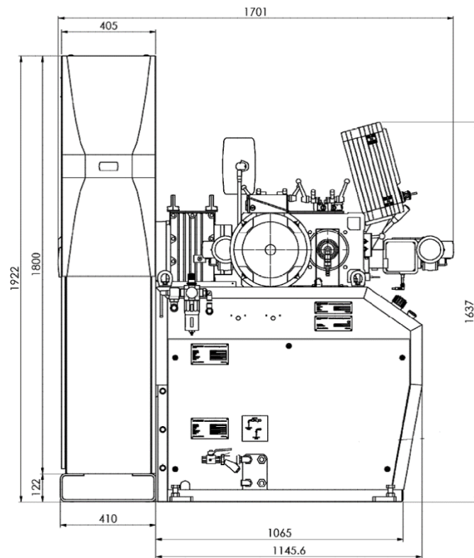
Front and Side view of RETRAXX 6011 (Actual layout may slightly differ)
